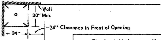
Shower Compartment 1024 sq. in.
