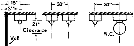
Stall and Wall Hung Urinals
