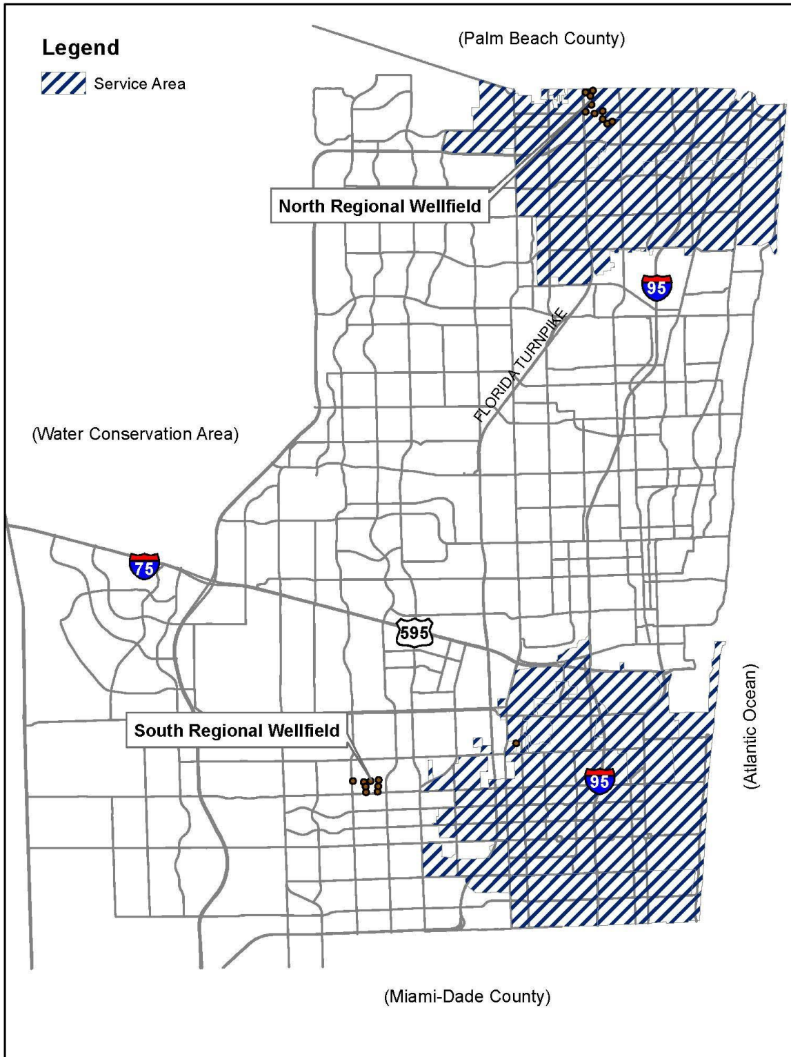
Figure 5-1. Regional Raw Water Service
