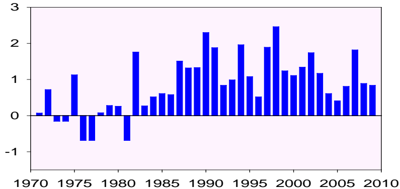
(A) Deviation of the Annual Avg Temperature (1F) in Ft. Lauderdale from the 1950-70 Baseline
